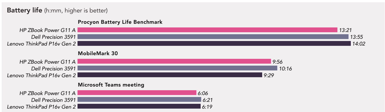
Figure 8: Battery life benchmark results in Windows 11 Best power efficiency power mode. More time is better. Source: Principled Technologies.
